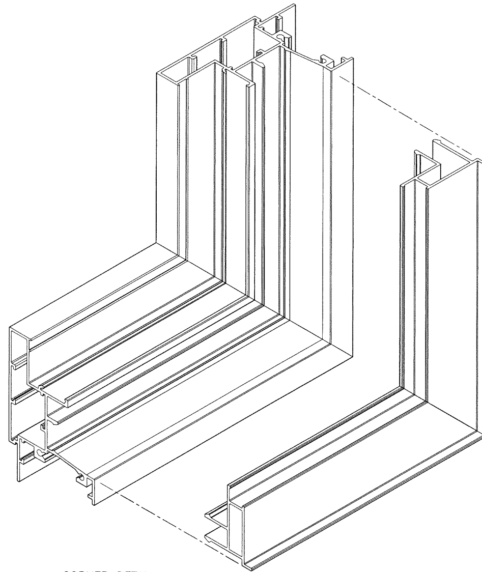
CORNER DETAIL INTERIOR VIEW
