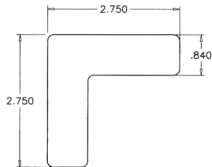
6 CORNER KEY TYPE 'A'
