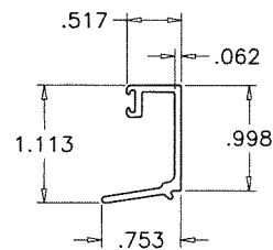
5 GLAZING BEAD 5/16" LAM. GLASS
