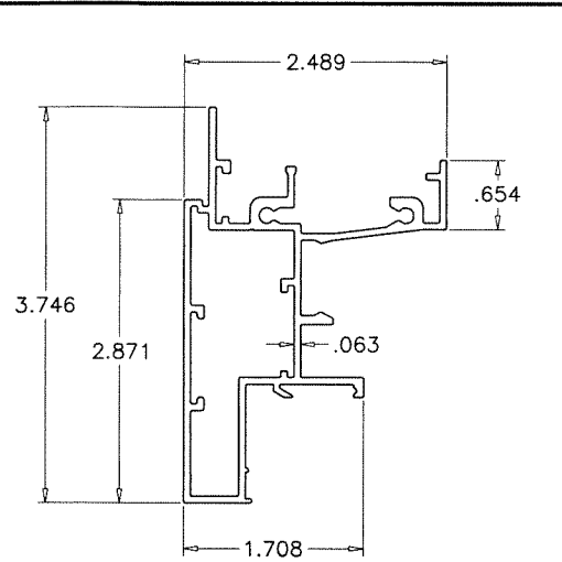
1 WINDOW FRAME
