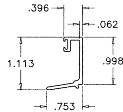
5A GLAZING BEAD 7/16" LAM. GLASS
